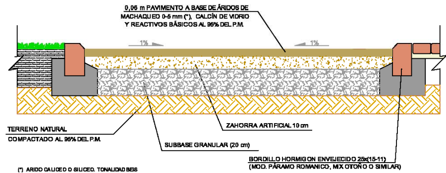
DETALLE 4 E:1/20
