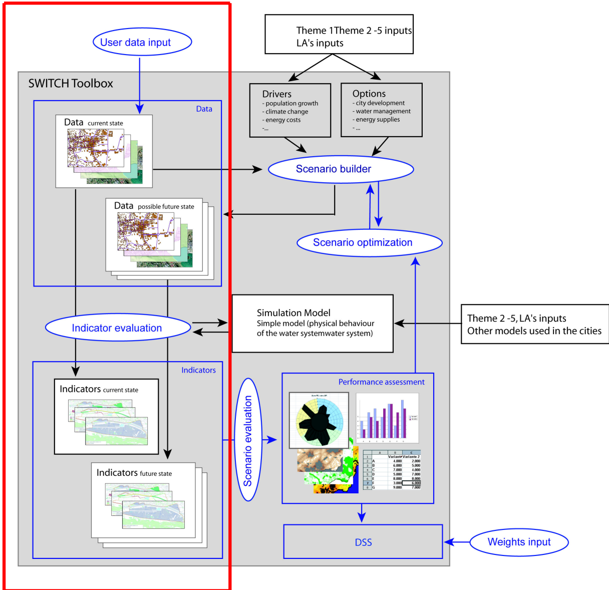
Figure 3.4: General features of the SWITCH toolbox and its relation with SMURF (Source: Adapted from Soutter 2007).
